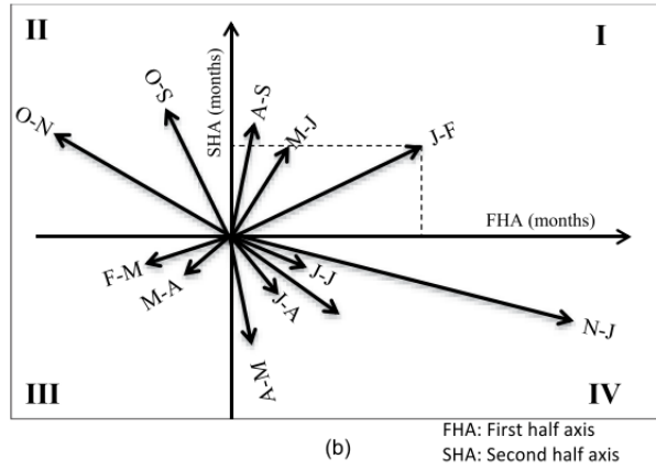
Figure 3: TPSC example [21]
