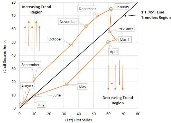
Figure 2: An innovative polygonal trend analysis (IPTA) template [22]
