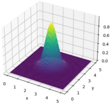
Wave Equation at time 0.40
