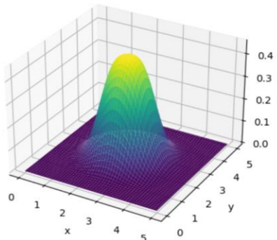
Wave Equation at time 0.40
