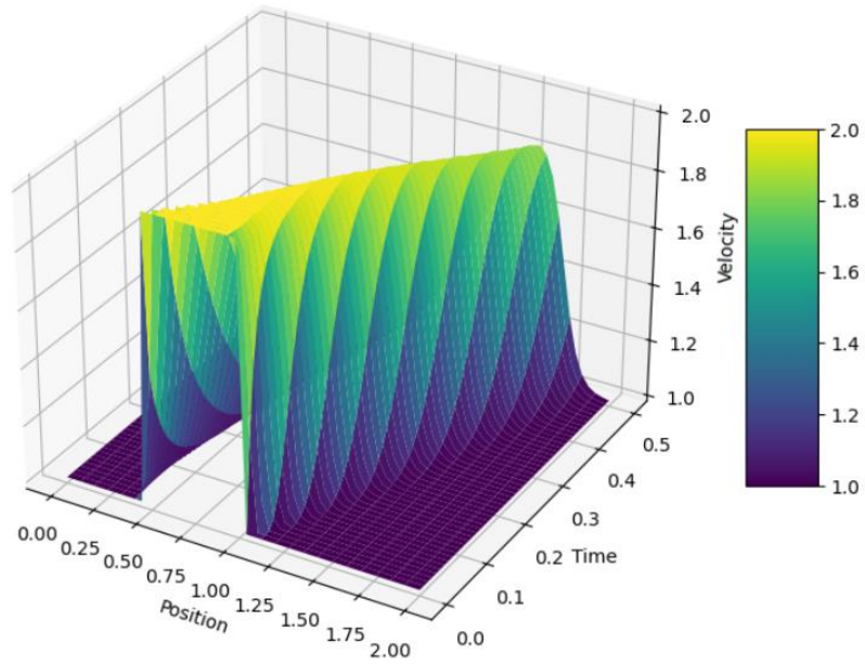
Burgers' Equation Solution Over Time
