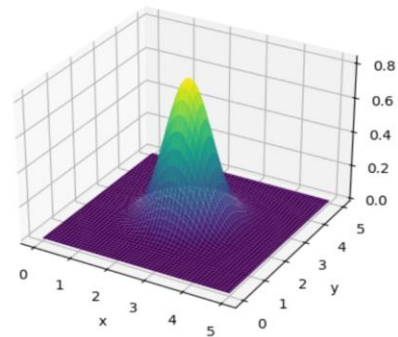
Wave Equation at time 0.20
