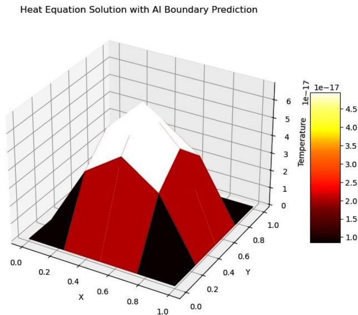
Figure 1: Graphic presentation of Heat Equation with Finite Difference Methods
