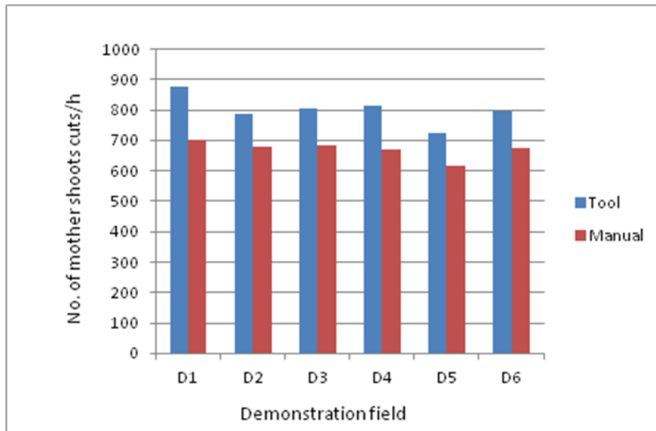
Fig.4: Performance of sugarcane mother shoot cutter
