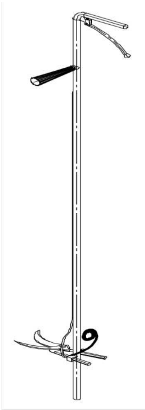
Fig. 1: Manually operated sugarcane mother shoot cutter
