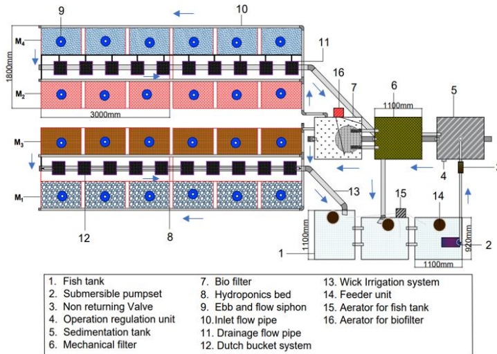
Fig.1. The schematic representation of system
