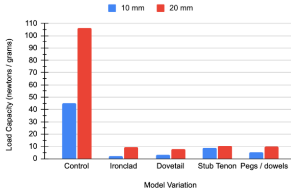
Fig. 5 : summarized bar graphs for each non-control breakboard, displaying the maximum load threshold value for each board variation
