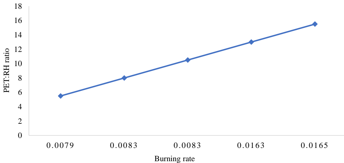
Figure 1 Variation of PET: RH ratios with burning rate at constant PET.
