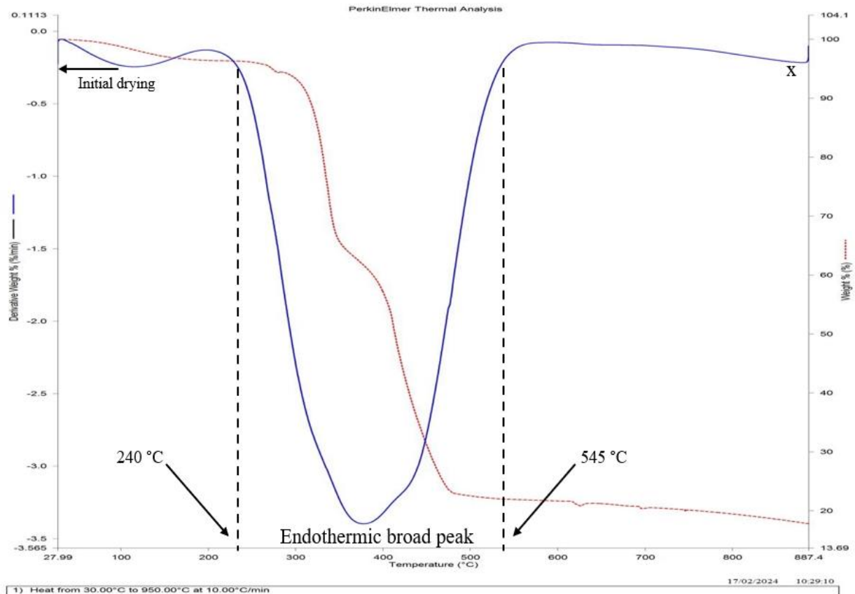
Figure 4 Differential thermal graph of the PET:RH composite (DTG)
