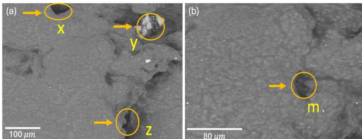
Figure 5 Scanning electron micrograph showing the surface morphology of the PET-RH composite at: 500× (a) and 1000× (b) magnification.
