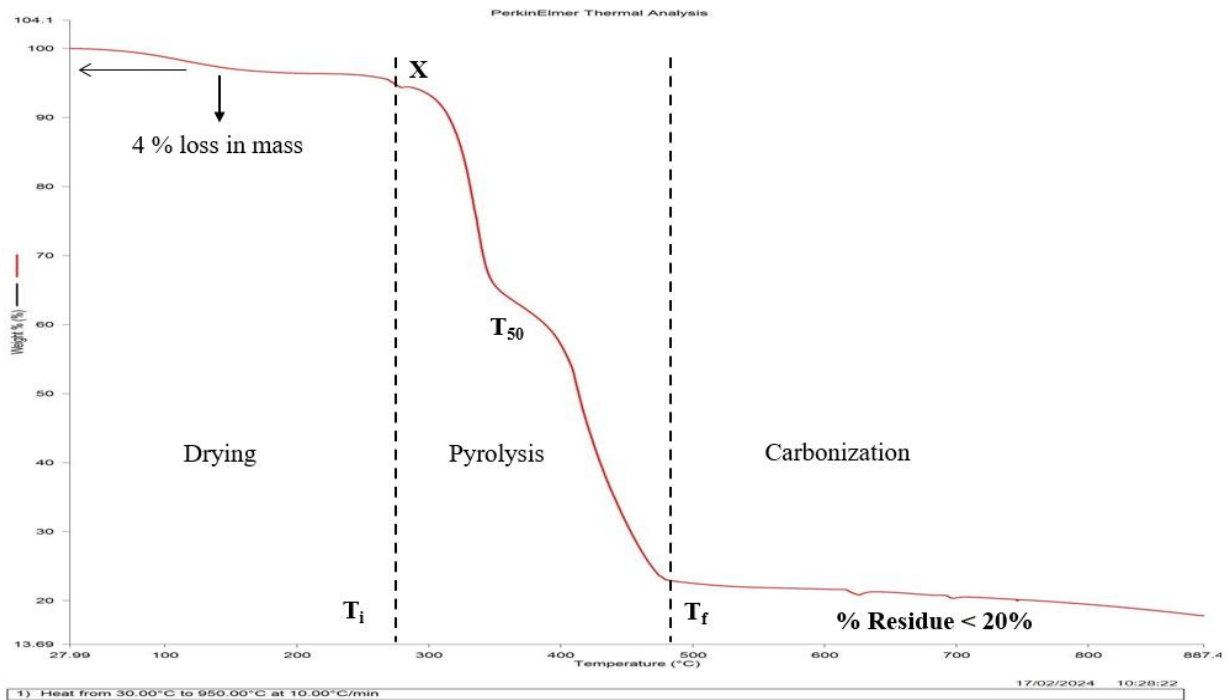
Figure 3 Thermogravimetric curve of PET: RH composite (TGA)
