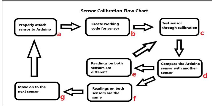
Fig 4: Diagram presents the flow chart of the sensor calibration procedures.
