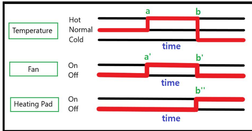
Fig 9: Diagram presents the response of the fan and heating pad to the temperature in the cat shelter.
