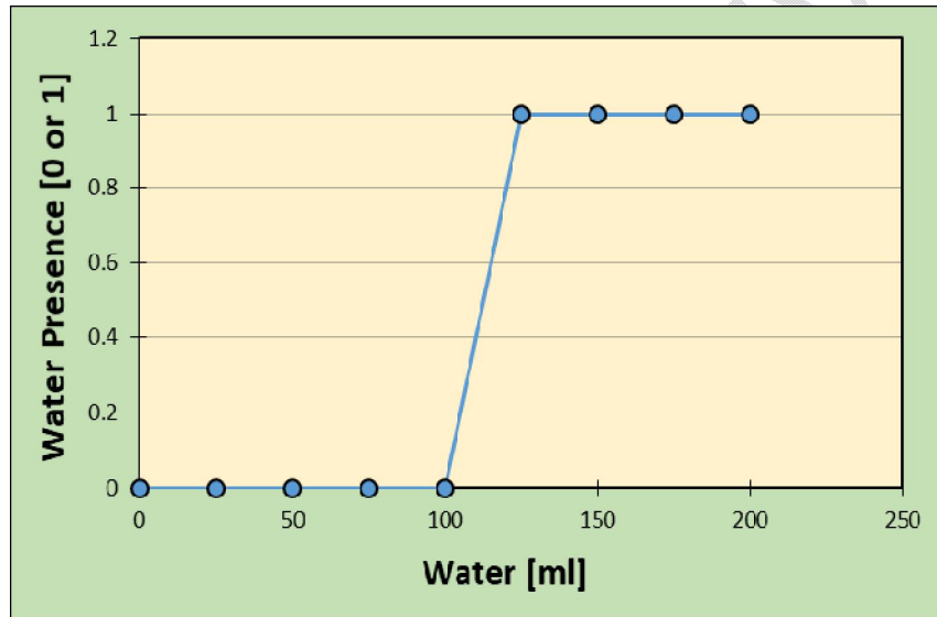
Fig. 8 illustrates the digital potential output from Arduino while changing the water level in the water supply container.
