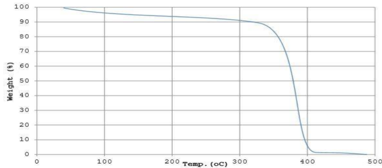
Figure 7: Graph of weight loss % versus Temperature.
