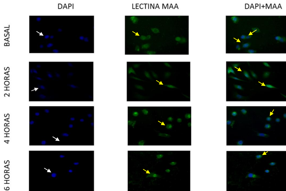
Figure 1 Effect of lipopolysaccharide (LPS) on \alpha 2,3-sialic acid expression in MCF-7 cells. MCF-7 cells were stimulated with LPS 20 ng/ml at 2, 4 and 6 hours, then incubated with Maackia amurensis lectin (MAA), and finally MCF-7 cells were stained with DAPI (4',6-diamidino-2-phenylindole) to mark nuclei, which are shown in blue. The first column of the image shows the DAPI-labelled nuclei, the second column shows the lectin labeling in green and the third column shows the colocalization. The white arrow indicates nucleus recognition. The yellow arrow indicates lectin recognition. Micrographs at 40X.
