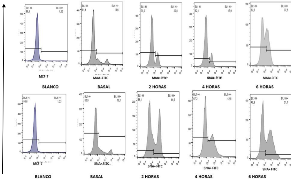
Figure 3 Effect of LPS on \alpha 2,3 and \alpha 2,6 sialic acid expression in the breast cancer cell line MCF-7 by flow cytometry. MCF-7 cells were treated with 20 ng/ml LPS for 2,4 and 6 h. Control and treated cells were incubated for 1.5 h under dark conditions with FITC-conjugated Maackia amurensis (MAA) lectin and FITC-conjugated Sambucus nigra (SNA) at 5 \mu g/ml. In A results for the expression of \alpha 2,3 sialic acid recognized by Maackia amurensis lectin (MAA). 18.6% of the population expressed sialic acid in unstimulated cells, while at 2 hours 20.8% of the cells expressed sialic acid, at 4 hours 18% the cells expressed sialic acid and at 6 hours 37.5% of the cells expressed sialic acid. In B 19.1% of the population expressed sialic acid in unstimulated cells, while at 2 hours 44.9% of the cells expressed sialic acid, at 4 hours 42.8% of the cells expressed sialic acid, and at 6 hours 51.1% of the cells expressed sialic acid. The results are from a representative experiment of three independent experiments.
