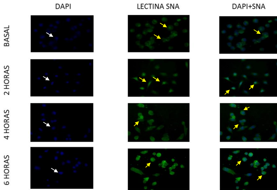
Figure 2 Effect of lipopolysaccharide (LPS) on \alpha 2,6-sialic acid expression in MCF-7 cells. MCF-7 cells were stimulated with LPS 20 ng/ml at 2.4 and 6 hours, then incubated with Sambucus nigra lectin (SNA), and finally MCF-7 cells were stained with DAPI (4',6-diamidino-2-phenylindole) to mark nuclei, which are shown in blue. The first column of the image shows the DAPI-labelled nuclei, the second column shows the lectin labeling in green and the third column shows the colocalization. The white arrow indicates nucleus recognition. The yellow arrow indicates lectin recognition. Micrographs at 40X.
