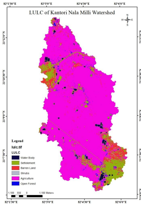
Fig. 4: LULC map of the study mili watershed
