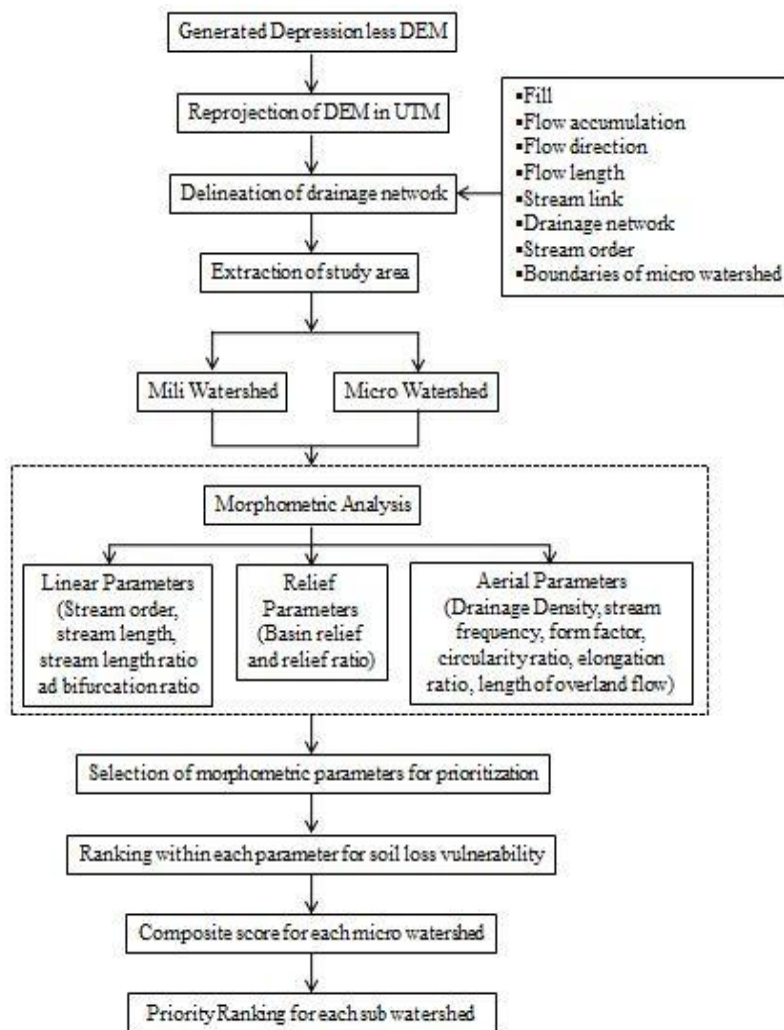
Fig. 2: Flowchart of methodology used in morphometric analysis
